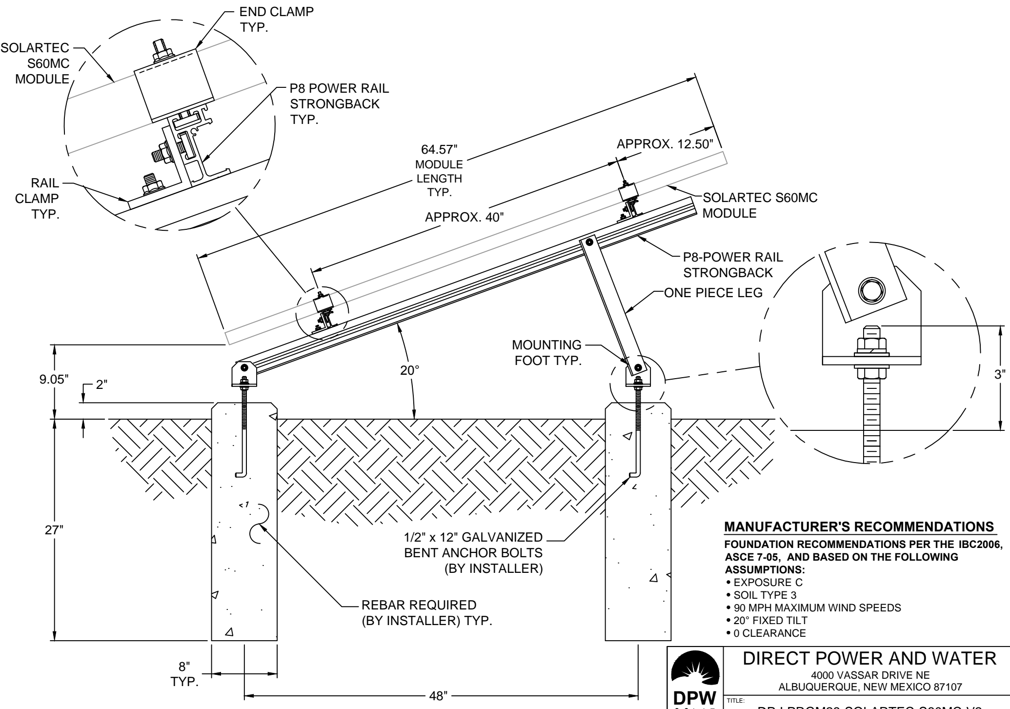
SIDE VIEW
